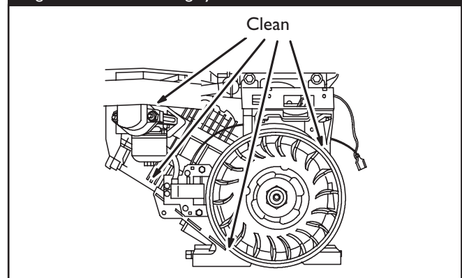
Figure 13 — Air Cooling System
